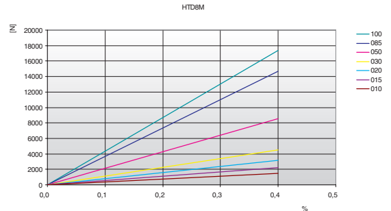
Load / Elongation [ % ]
