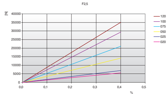
Load / Elongation [ % ]
