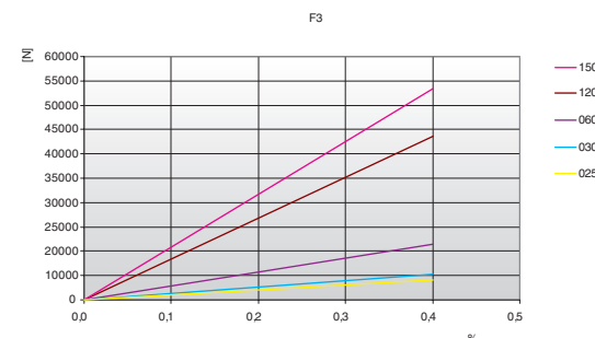
Load / Elongation [ % ]
